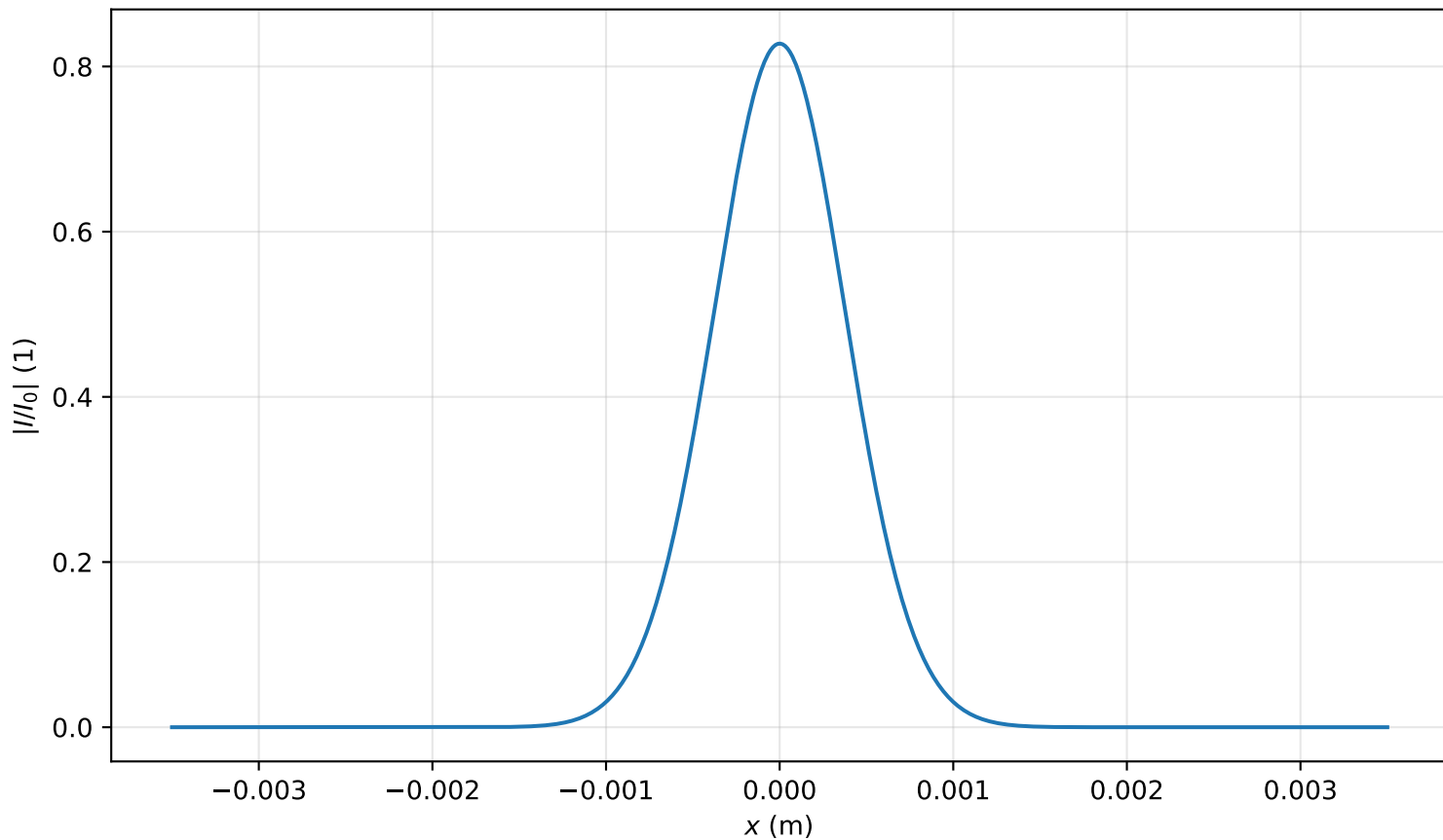
Intensity profile I(x, y = 0, z = 1.035m)/I_0 , P_{in}=0.1P_{cr} , artificial time
